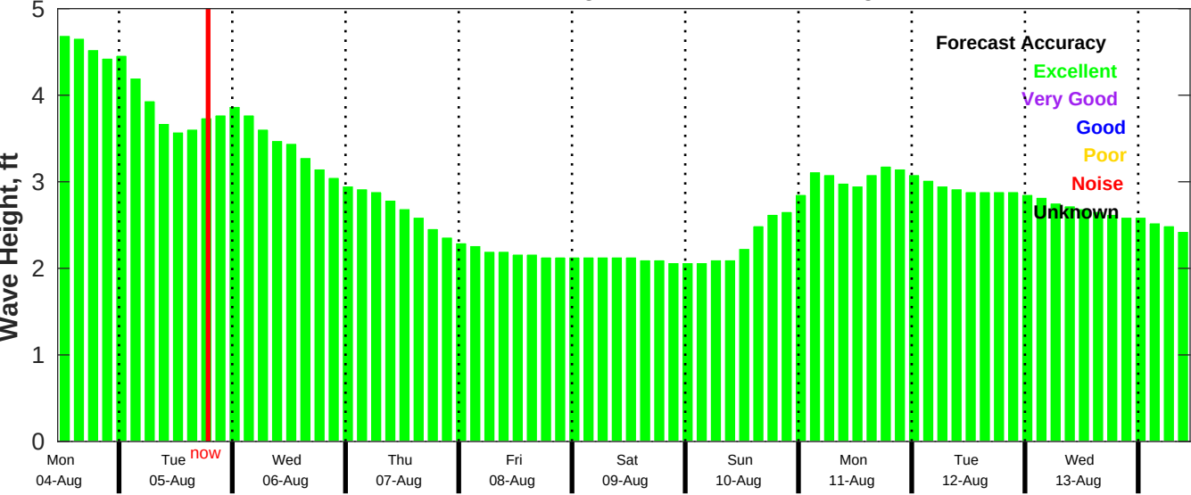
CMEMS Wave Forecast for NDBC 52211 from 03-Aug-2025 11:00:00 to 13-Aug-2025 11:00:00
