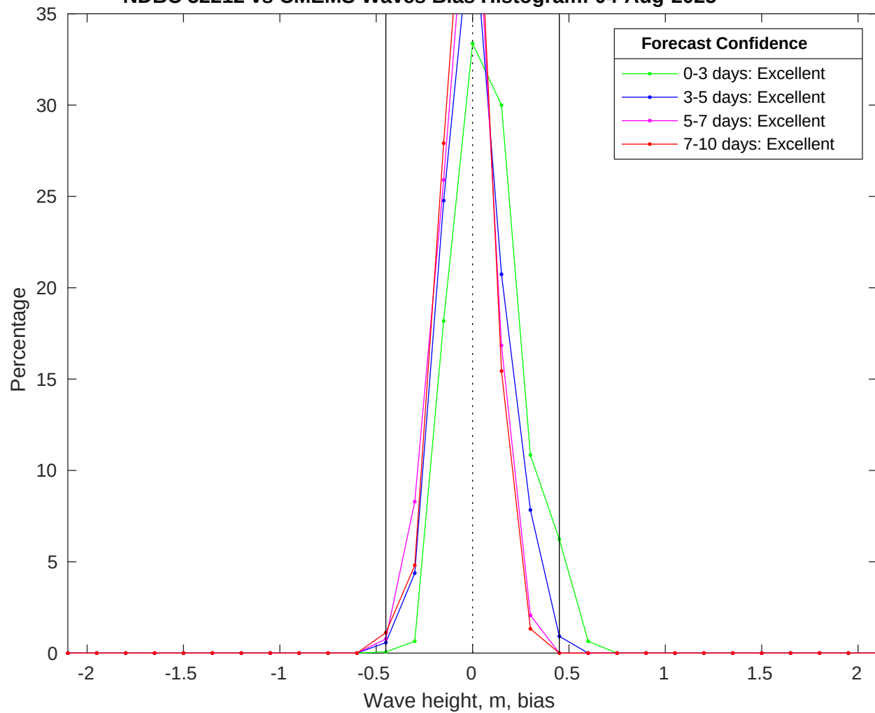
NDBC 52212 vs CMEMS Waves Bias Histogram: 04-Aug-2025
