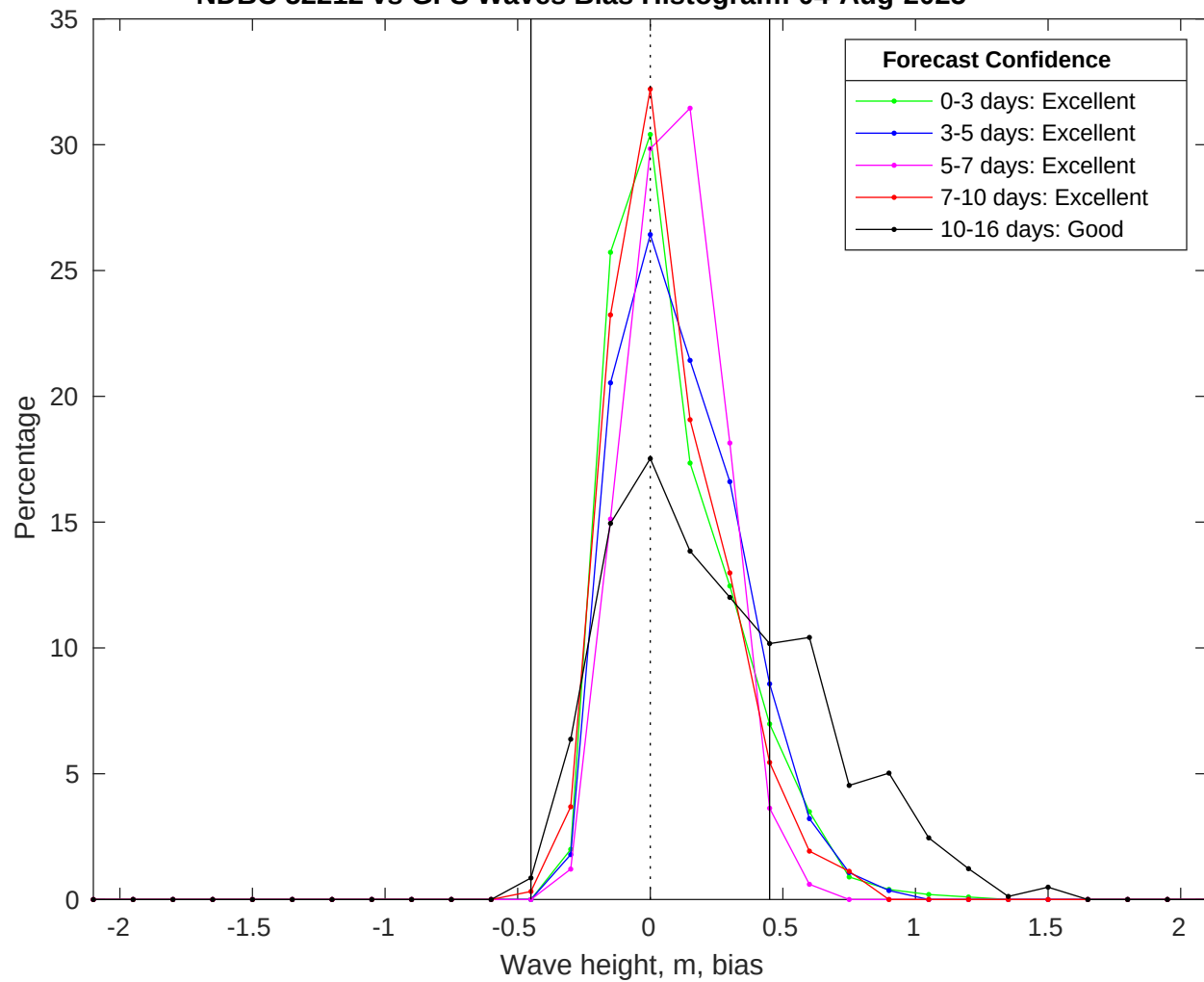
NDBC 52212 vs GFS Waves Bias Histogram: 04-Aug-2025
