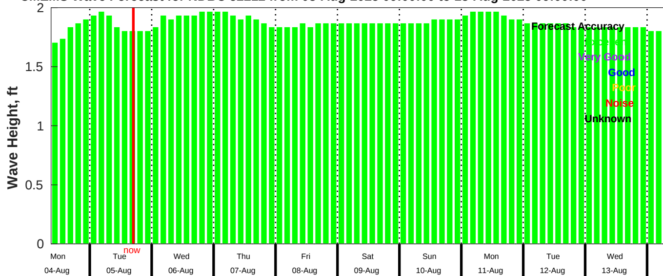
CMEMS Wave Forecast for NDBC 52212 from 03-Aug-2025 09:00:00 to 13-Aug-2025 09:00:00
