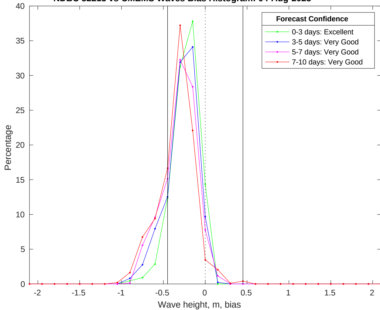
NDBC 52213 vs CMEMS Waves Bias Histogram: 04-Aug-2025
