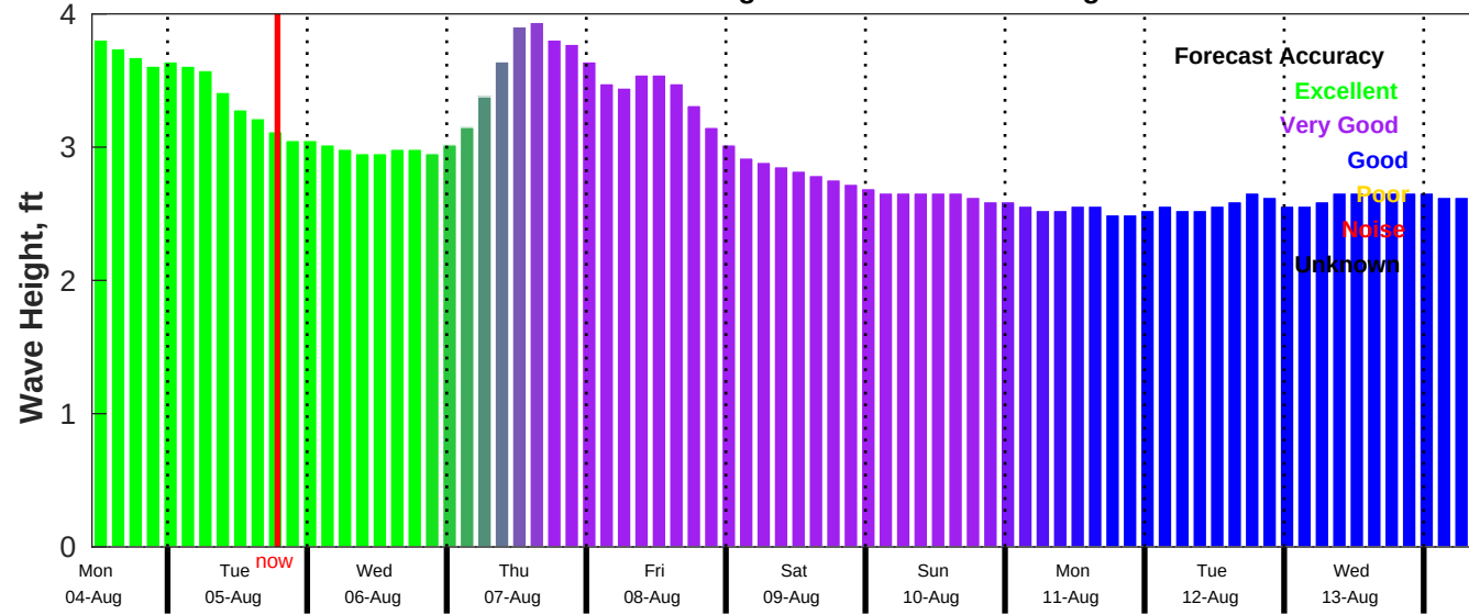
CMEMS Wave Forecast for NDBC 52213 from 03-Aug-2025 11:00:00 to 13-Aug-2025 11:00:00
