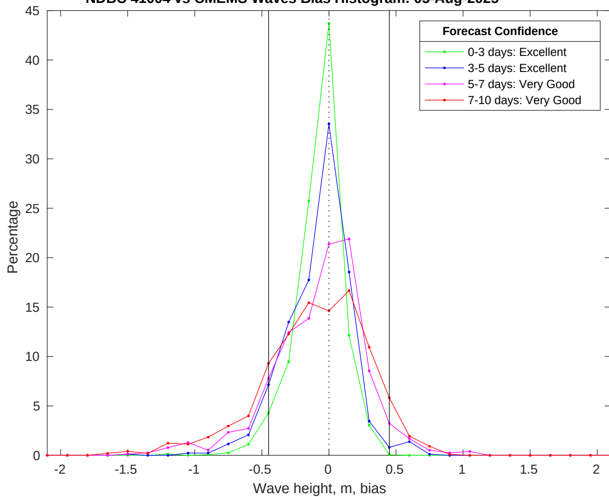
NDBC 41004 vs CMEMS Waves Bias Histogram: 05-Aug-2025
