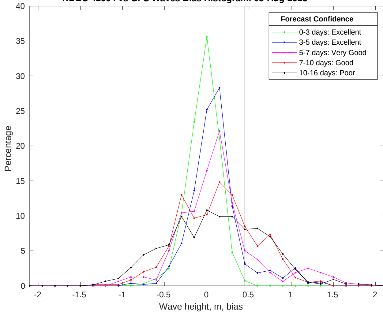
NDBC 41004 vs GFS Waves Bias Histogram: 05-Aug-2025
