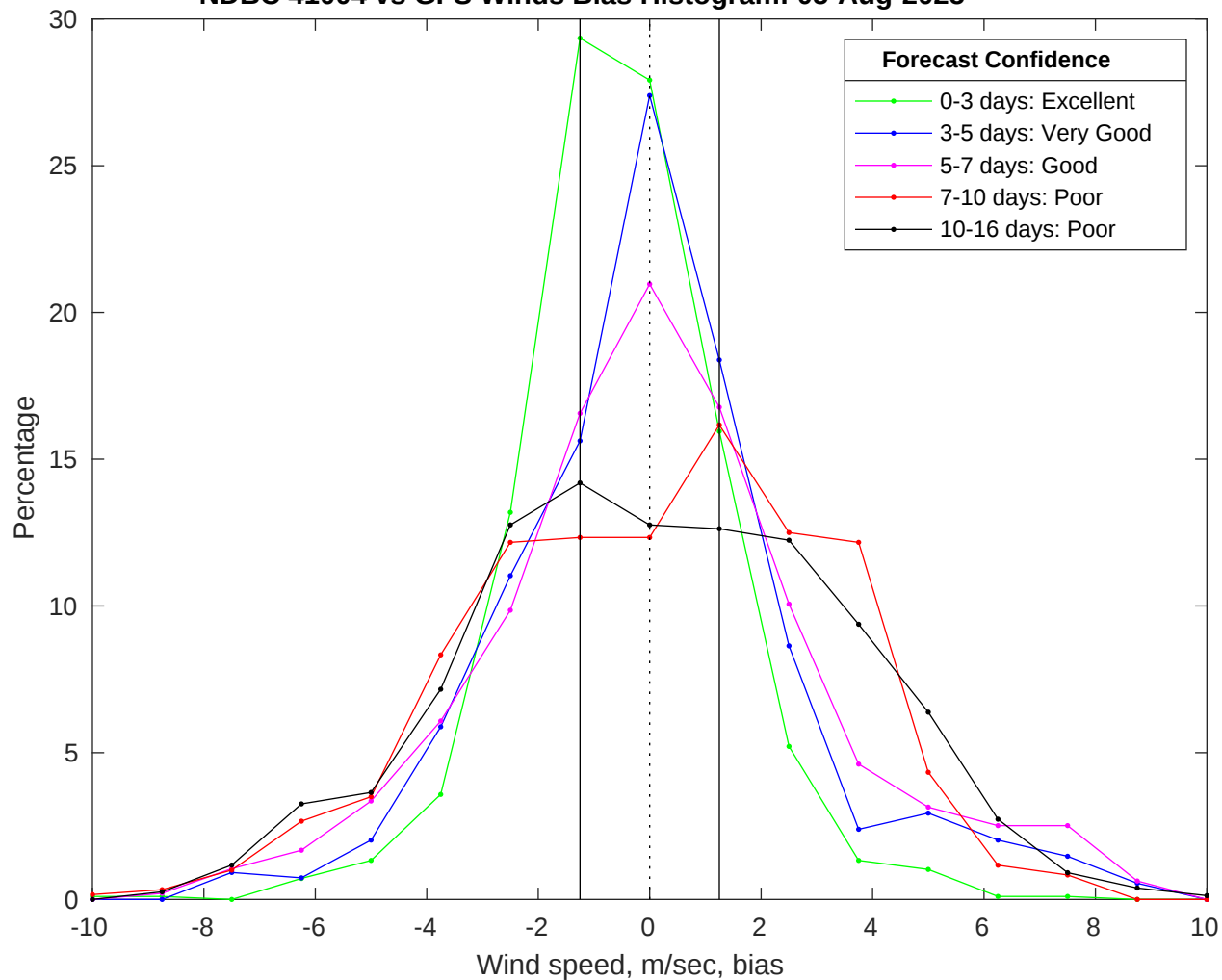
NDBC 41004 vs GFS Winds Bias Histogram: 05-Aug-2025
