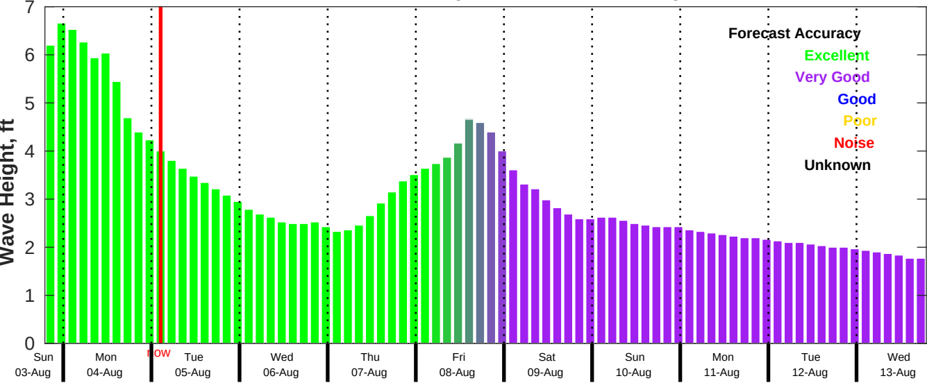
CMEMS Wave Forecast for NDBC 41004 from 03-Aug-2025 19:00:00 to 13-Aug-2025 19:00:00
