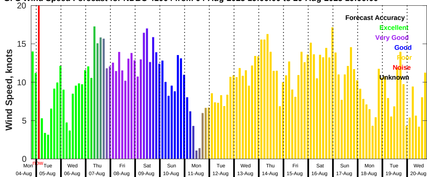
GFS Wind Speed Forecast for NDBC 41004 from 04-Aug-2025 19:00:00 to 20-Aug-2025 19:00:00
