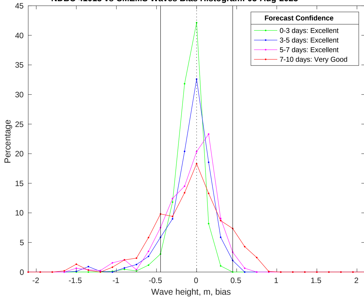
NDBC 41013 vs CMEMS Waves Bias Histogram: 05-Aug-2025
