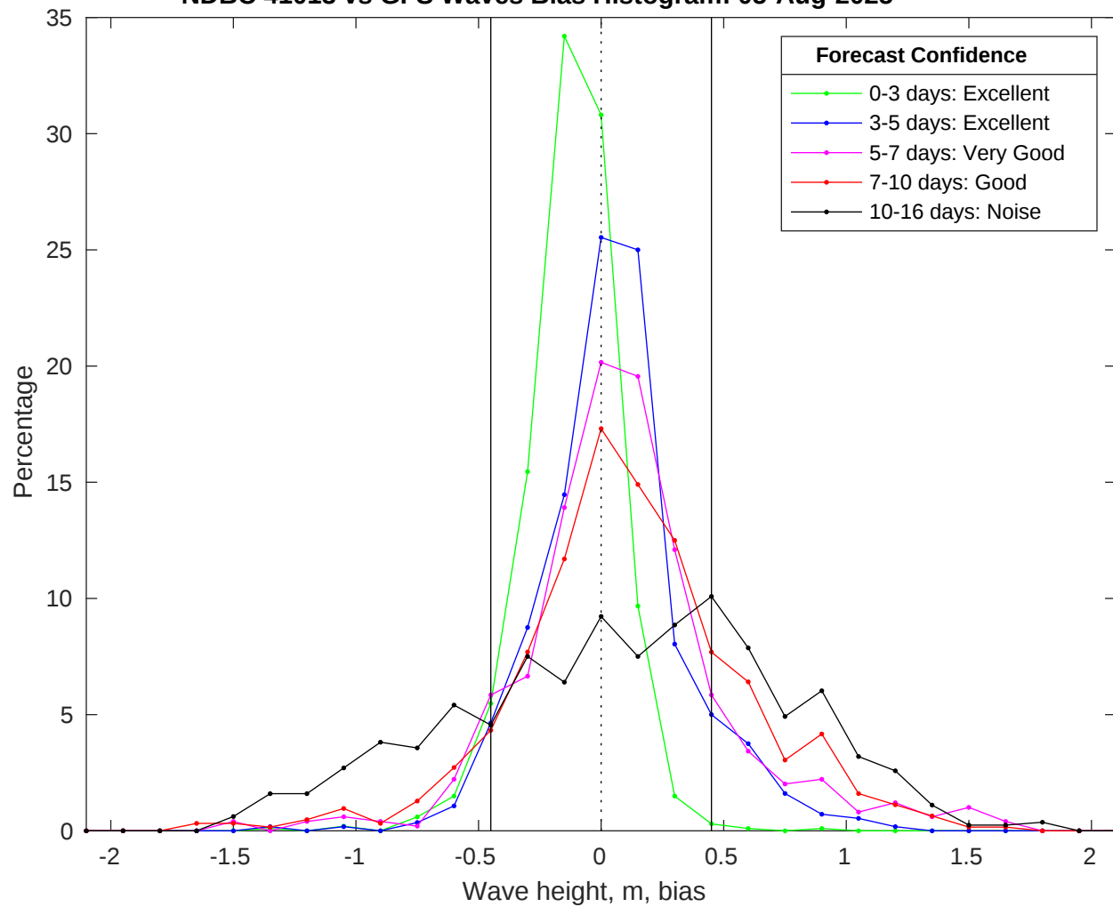
NDBC 41013 vs GFS Waves Bias Histogram: 05-Aug-2025
