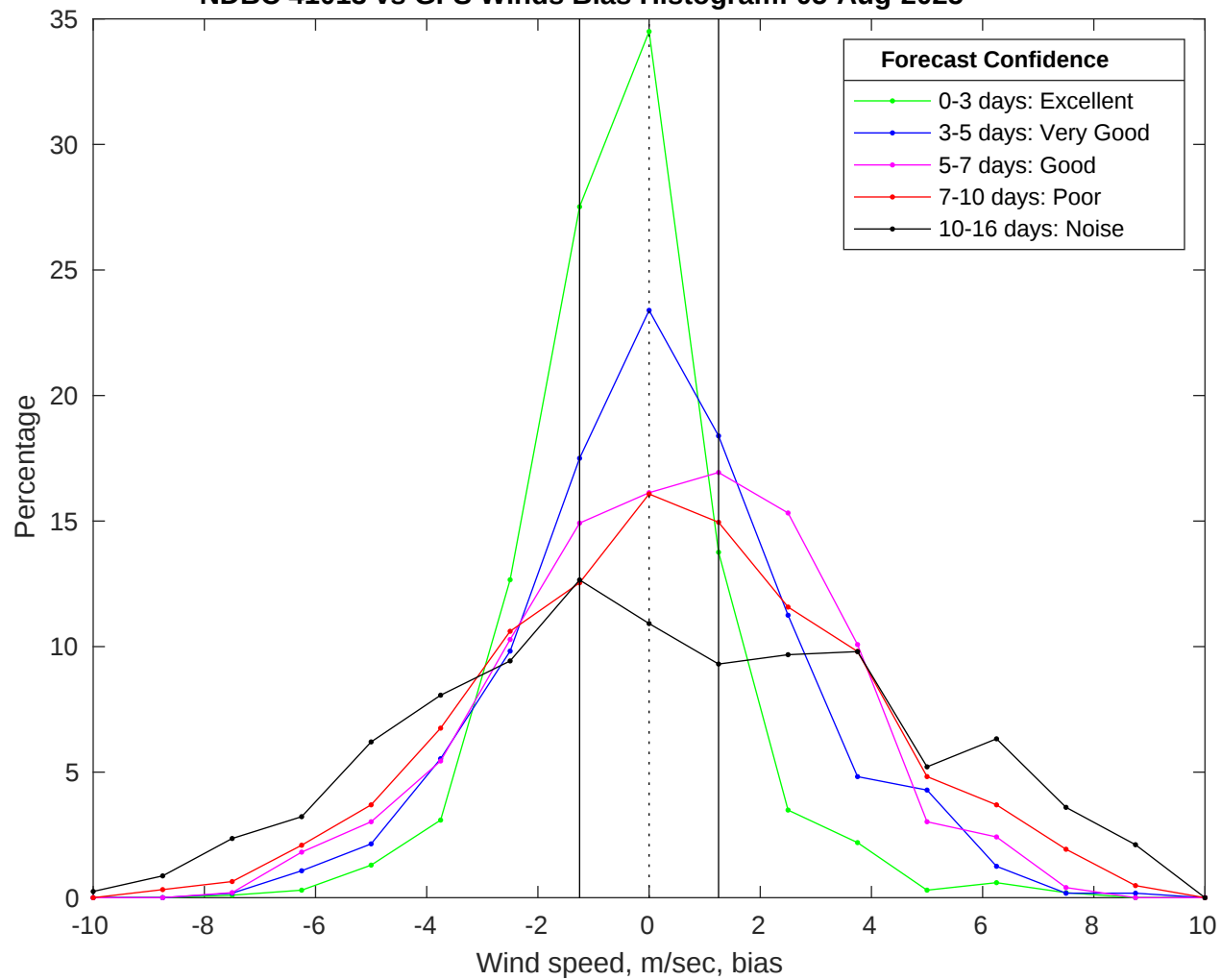
NDBC 41013 vs GFS Winds Bias Histogram: 05-Aug-2025
