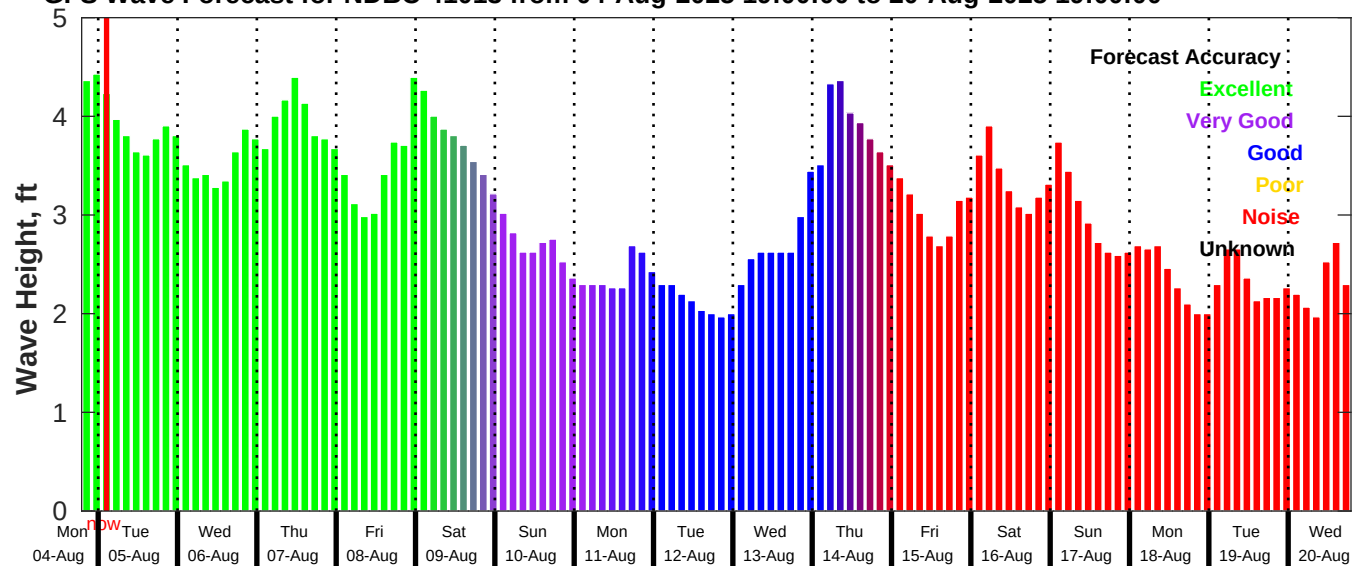
GFS Wave Forecast for NDBC 41013 from 04-Aug-2025 19:00:00 to 20-Aug-2025 19:00:00
