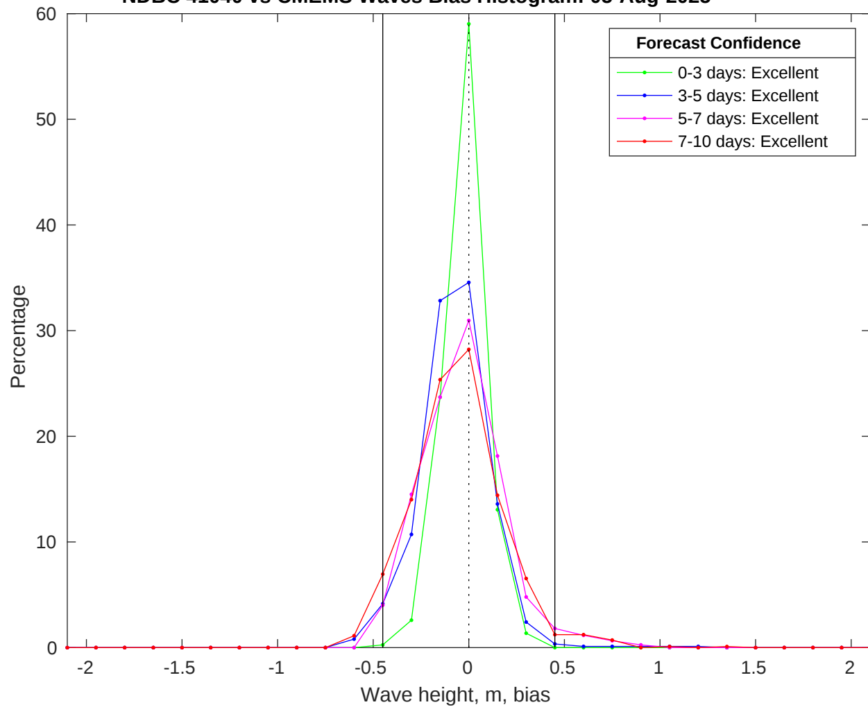
NDBC 41040 vs CMEMS Waves Bias Histogram: 05-Aug-2025
