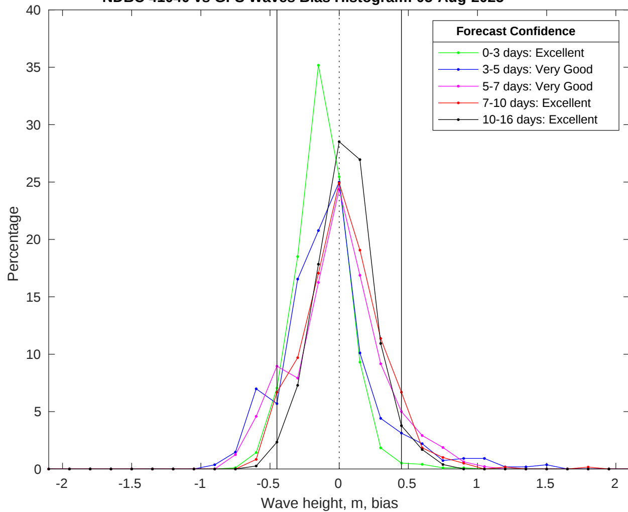
NDBC 41040 vs GFS Waves Bias Histogram: 05-Aug-2025
