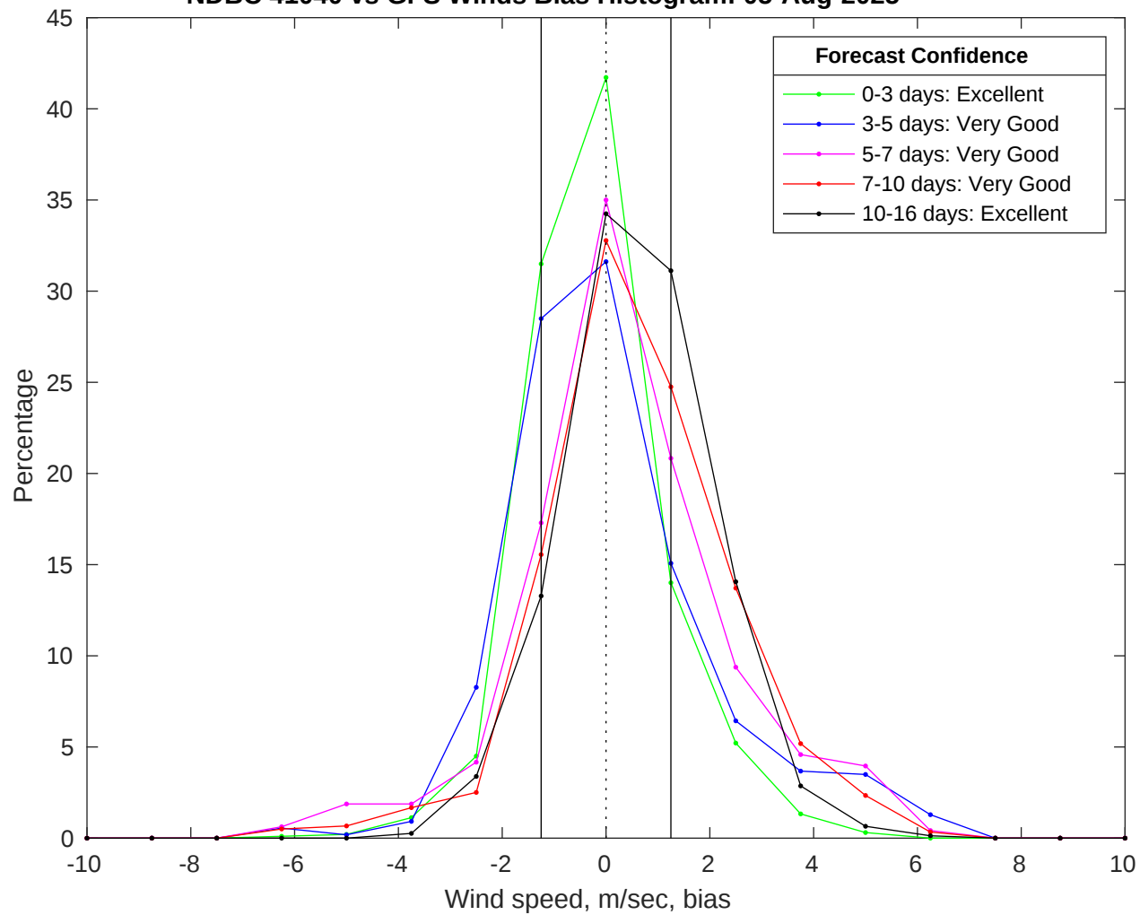
NDBC 41040 vs GFS Winds Bias Histogram: 05-Aug-2025
