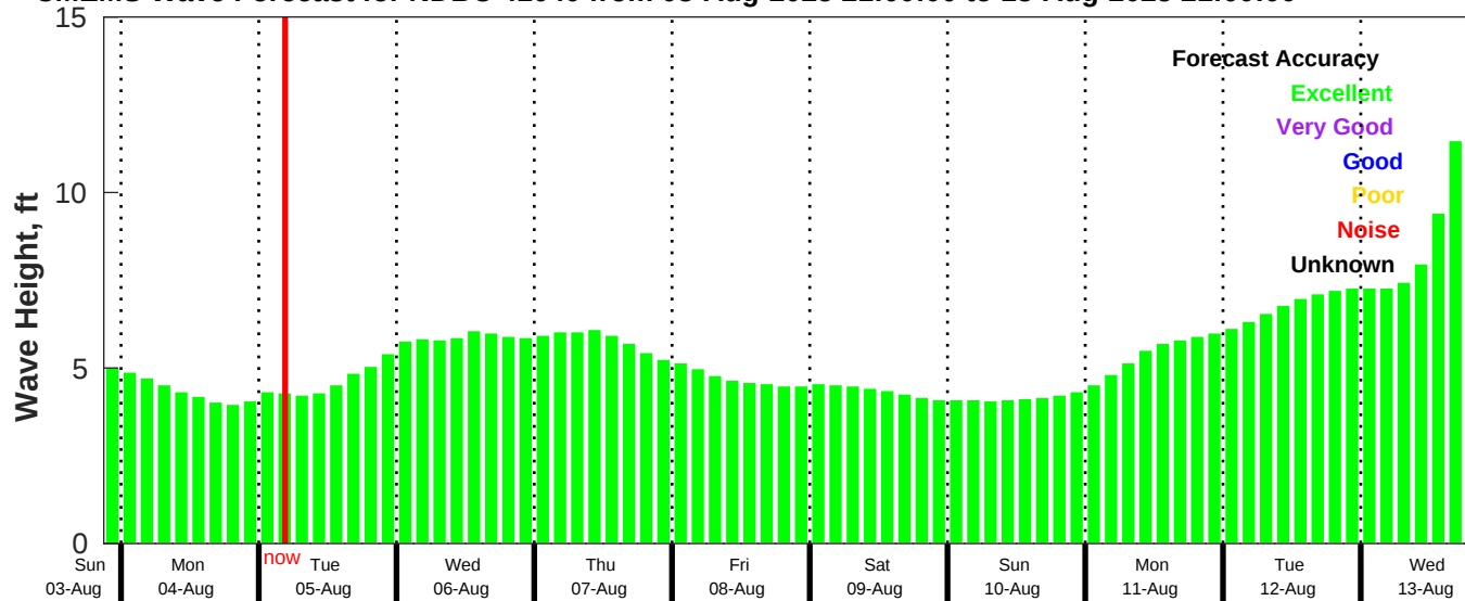
CMEMS Wave Forecast for NDBC 41040 from 03-Aug-2025 21:00:00 to 13-Aug-2025 21:00:00
