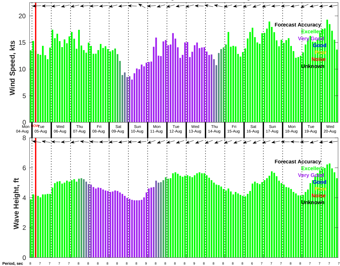
Wind & Wave Forecast for NDBC 41040 from 04-Aug-2025 21:00:00 to 20-Aug-2025 21:00:00
