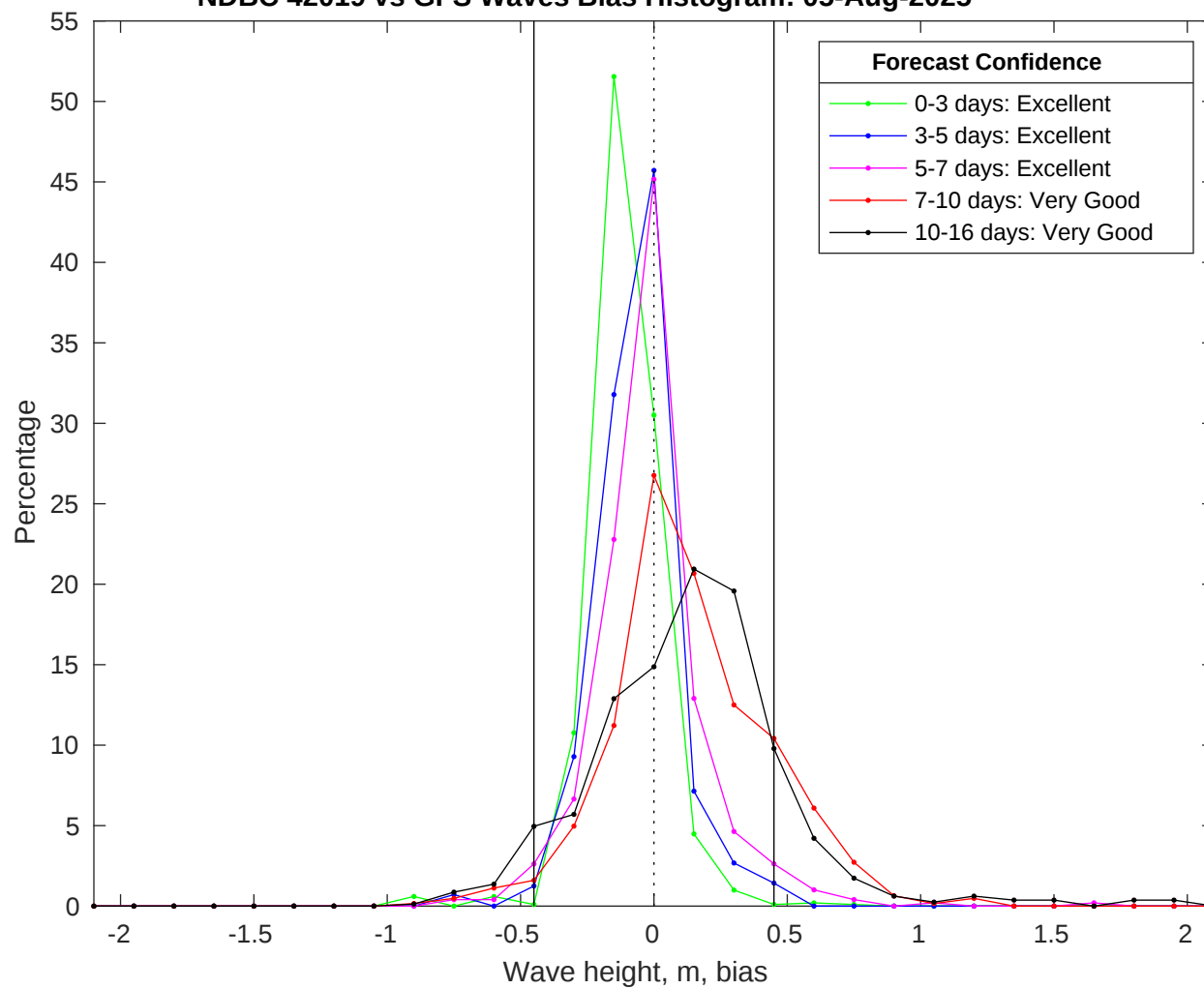
NDBC 42019 vs GFS Waves Bias Histogram: 05-Aug-2025
