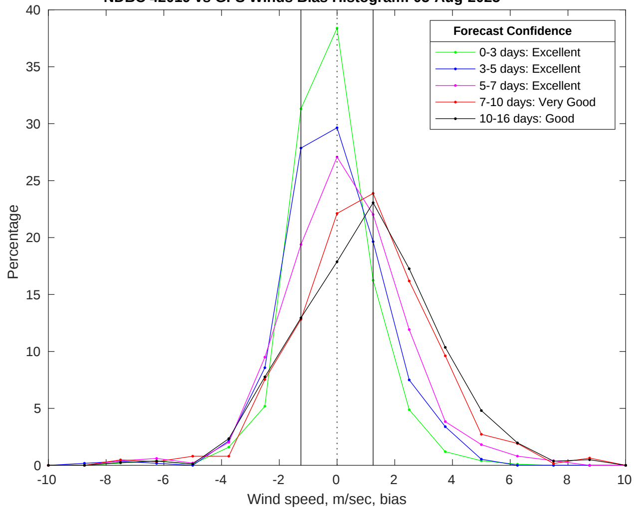
NDBC 42019 vs GFS Winds Bias Histogram: 05-Aug-2025
