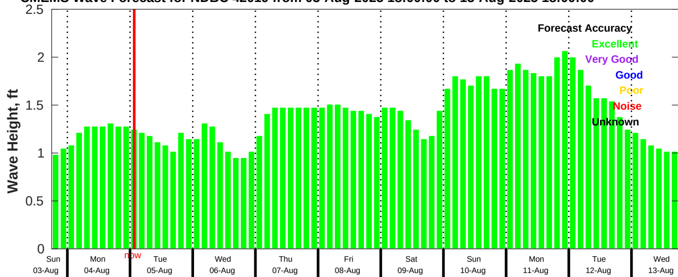
CMEMS Wave Forecast for NDBC 42019 from 03-Aug-2025 18:00:00 to 13-Aug-2025 18:00:00
