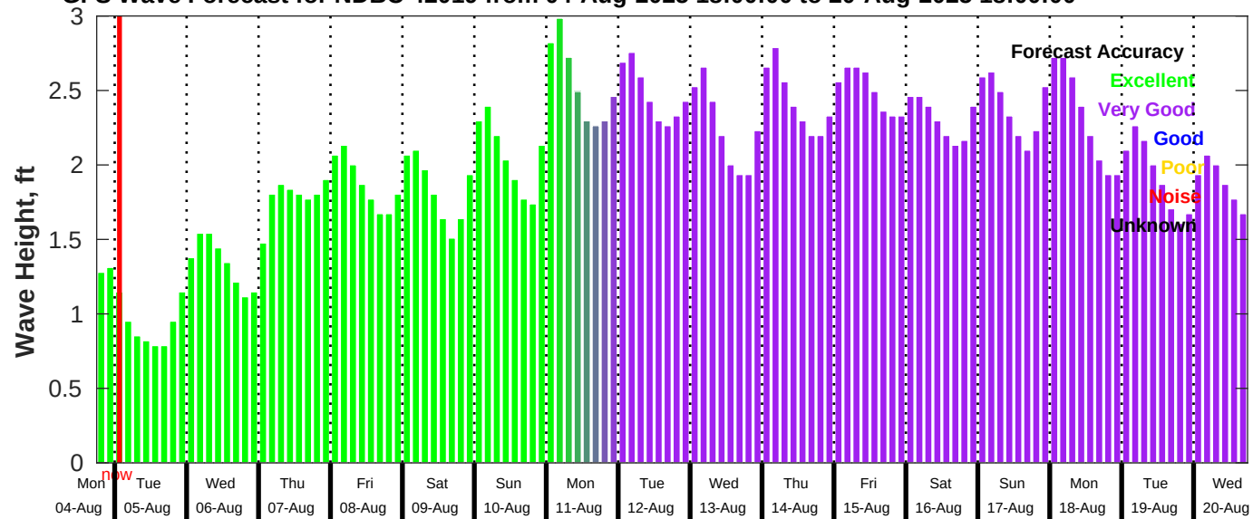
GFS Wave Forecast for NDBC 42019 from 04-Aug-2025 18:00:00 to 20-Aug-2025 18:00:00
