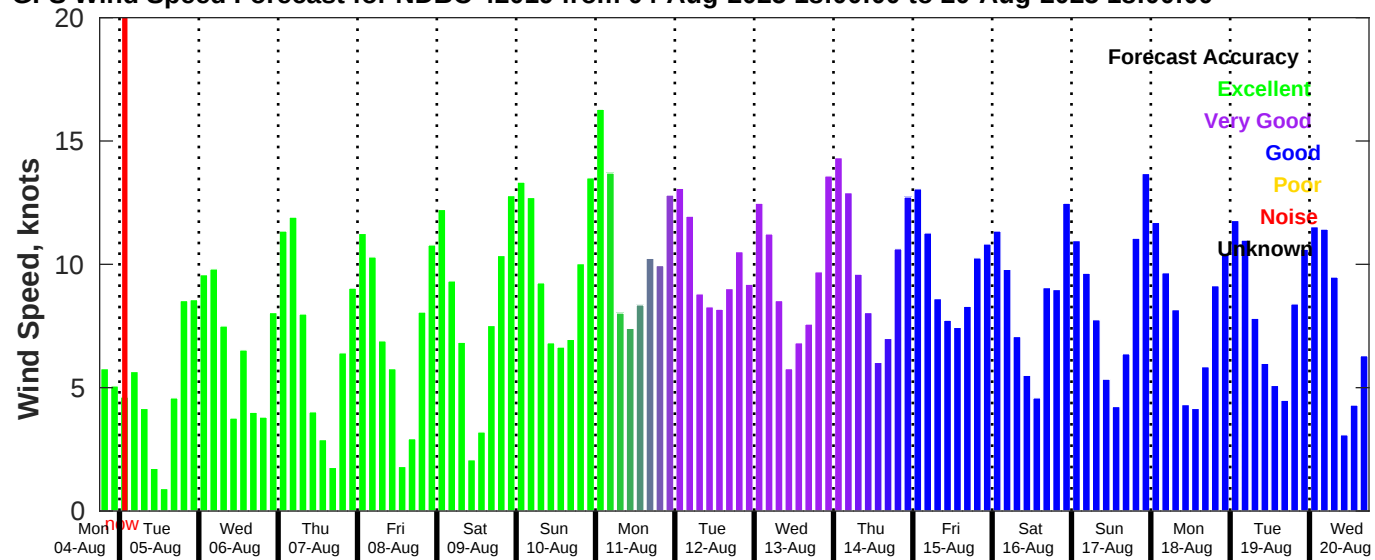
GFS Wind Speed Forecast for NDBC 42019 from 04-Aug-2025 18:00:00 to 20-Aug-2025 18:00:00
