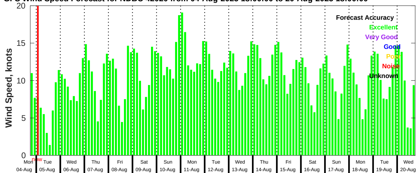
GFS Wind Speed Forecast for NDBC 42020 from 04-Aug-2025 18:00:00 to 20-Aug-2025 18:00:00
