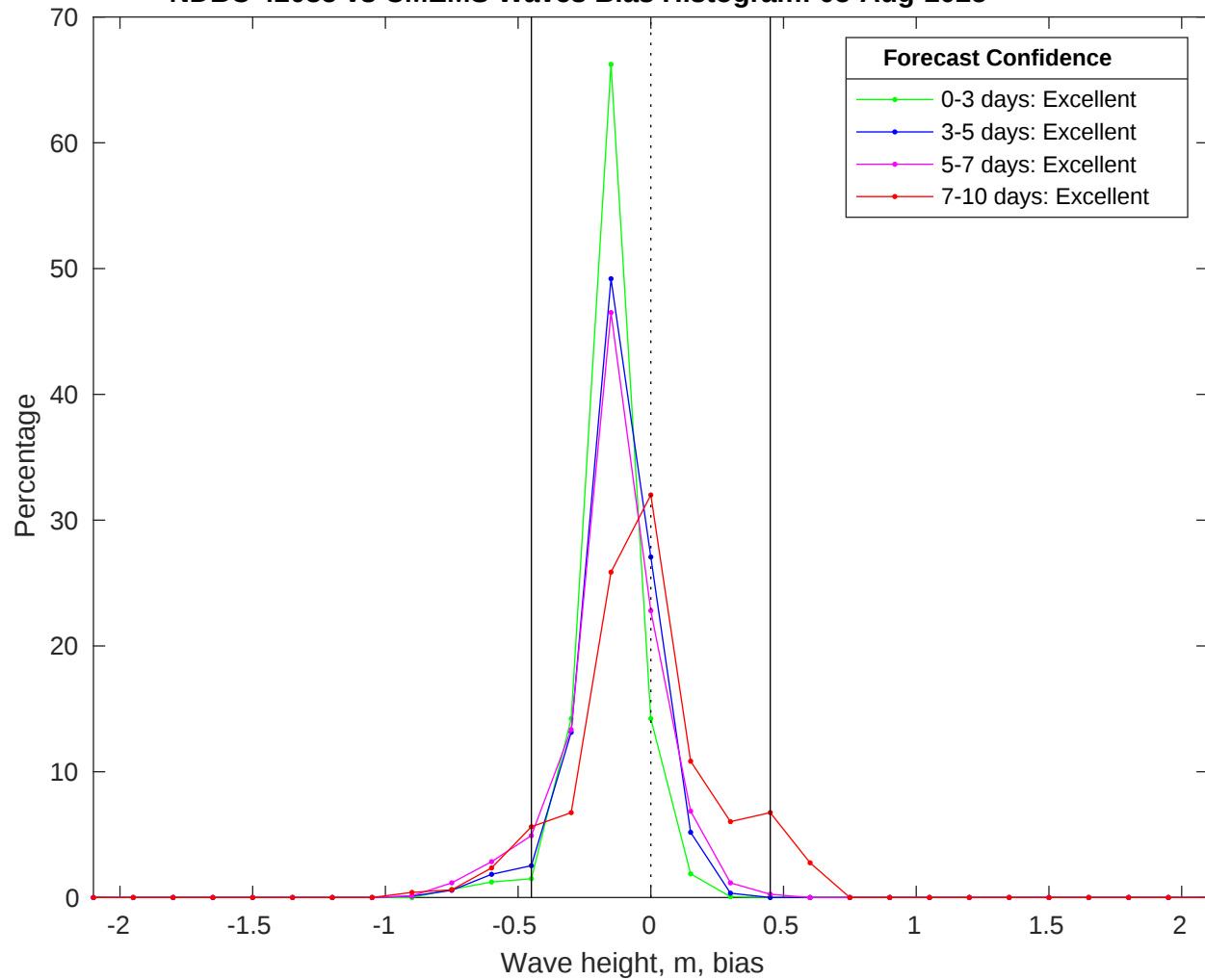
NDBC 42035 vs CMEMS Waves Bias Histogram: 05-Aug-2025
