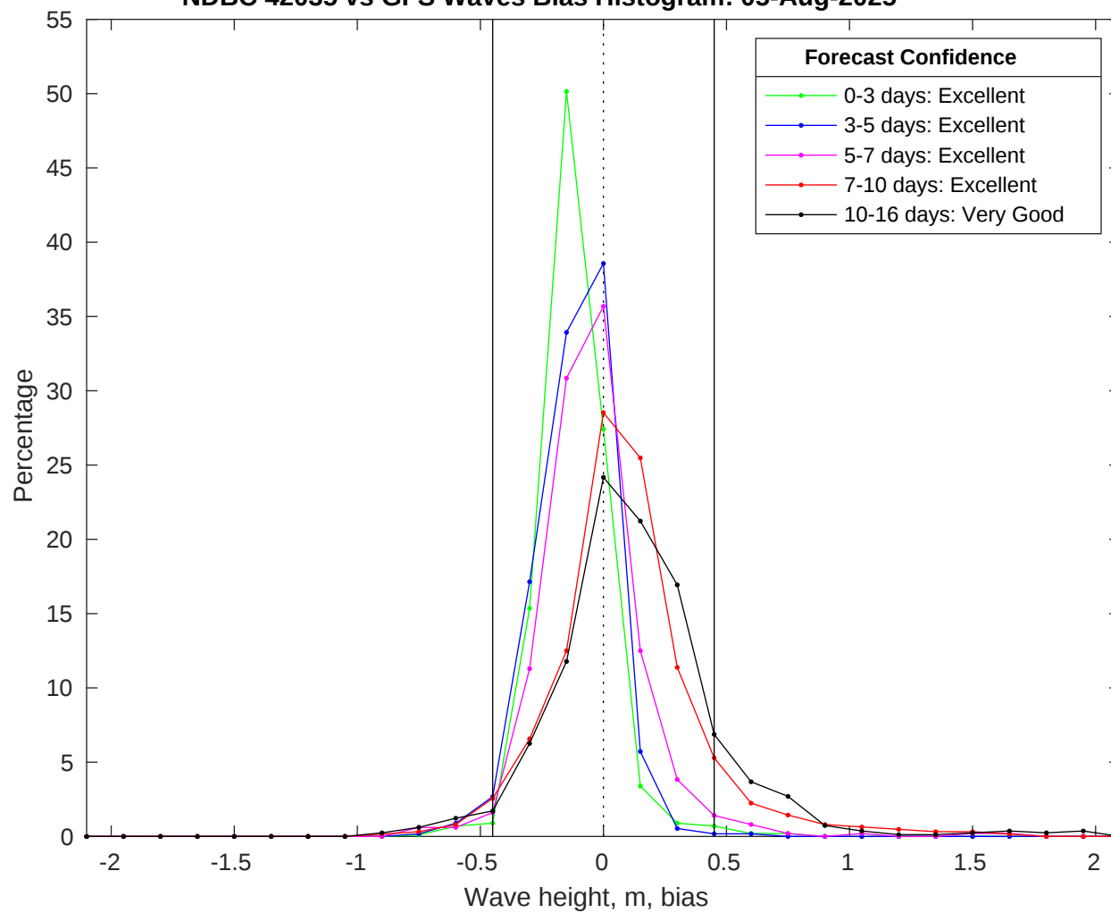
NDBC 42035 vs GFS Waves Bias Histogram: 05-Aug-2025
