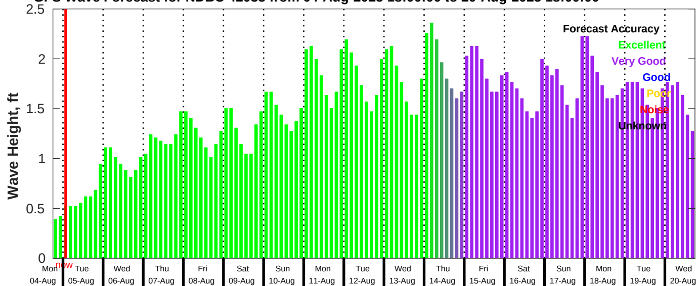
GFS Wave Forecast for NDBC 42035 from 04-Aug-2025 18:00:00 to 20-Aug-2025 18:00:00
