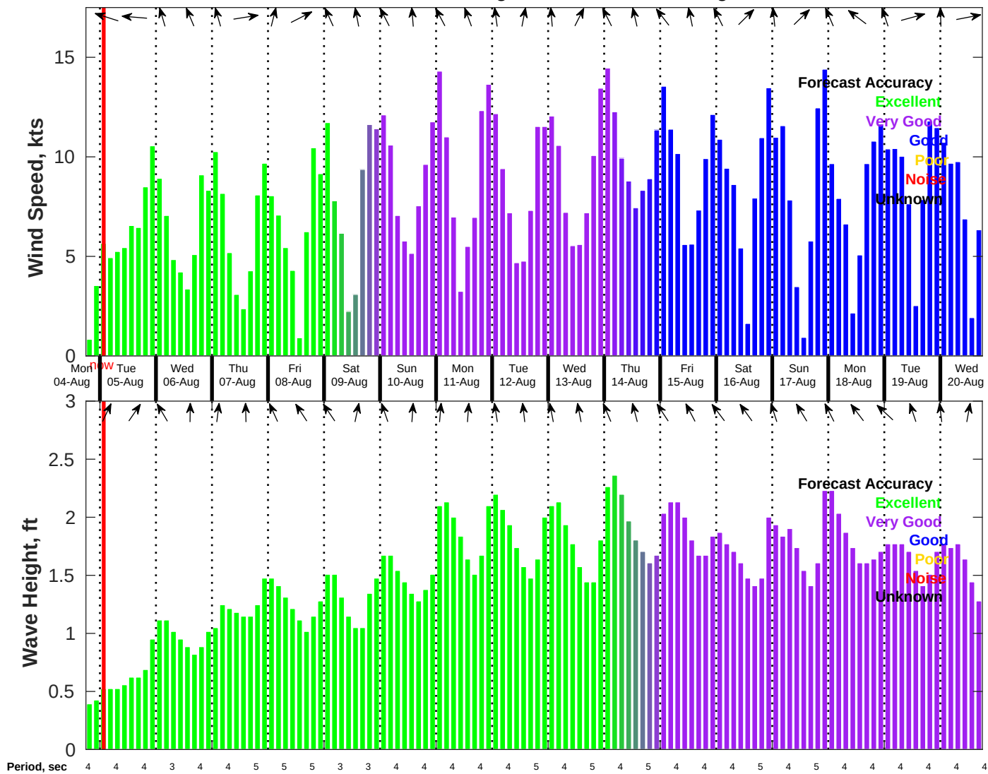
Wind & Wave Forecast for NDBC 42035 from 04-Aug-2025 18:00:00 to 20-Aug-2025 18:00:00
