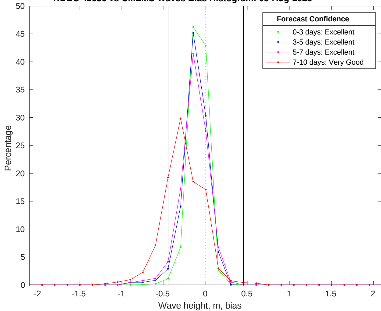
NDBC 42036 vs CMEMS Waves Bias Histogram: 05-Aug-2025
