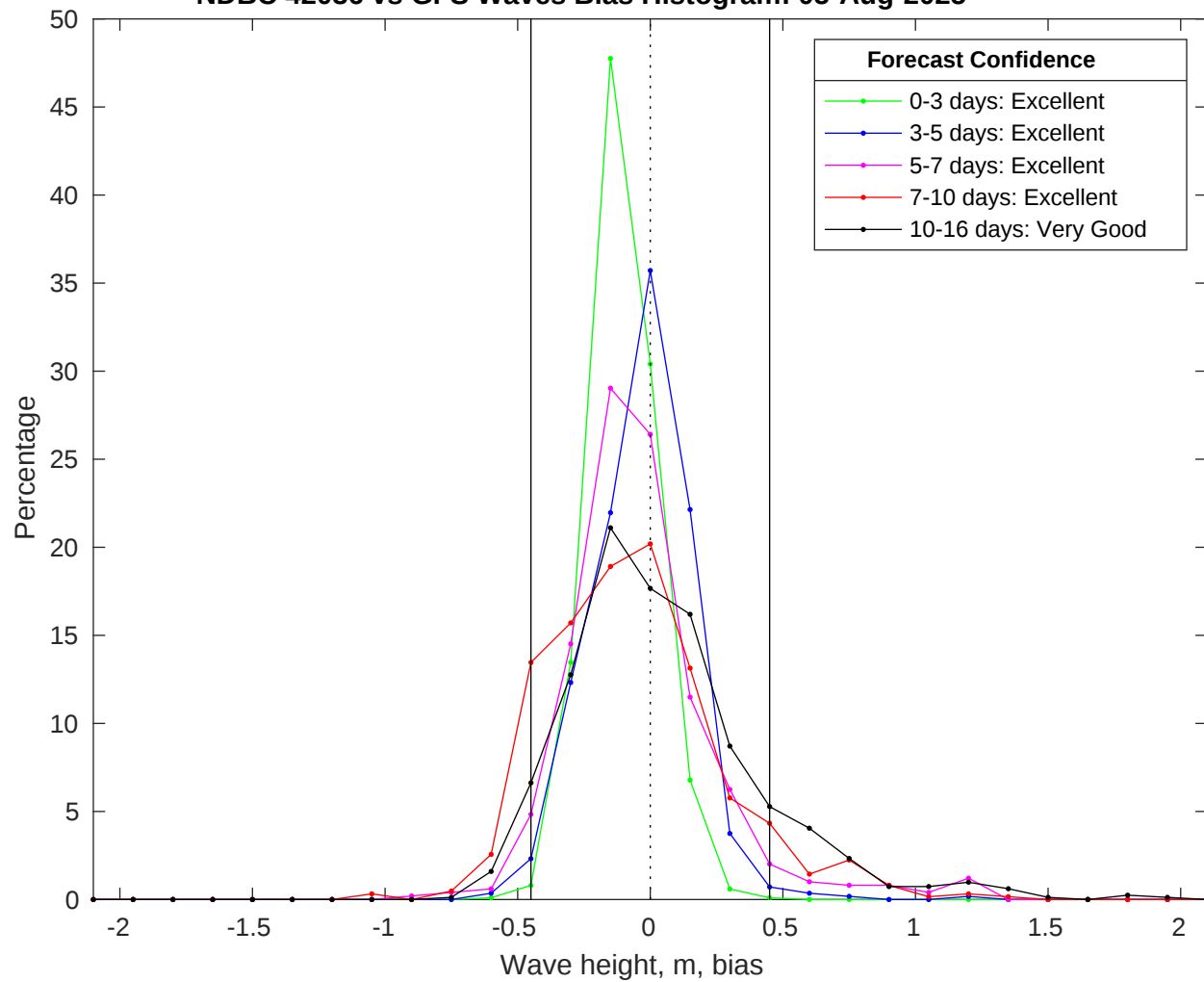
NDBC 42036 vs GFS Waves Bias Histogram: 05-Aug-2025
