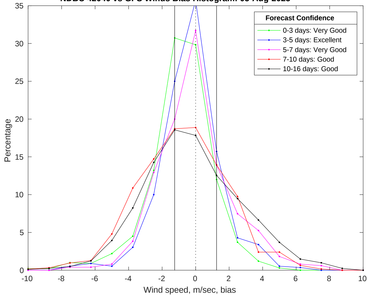
NDBC 42040 vs GFS Winds Bias Histogram: 05-Aug-2025
