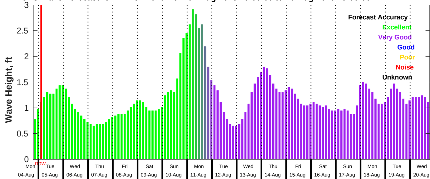
GFS Wave Forecast for NDBC 42040 from 04-Aug-2025 19:00:00 to 20-Aug-2025 19:00:00
