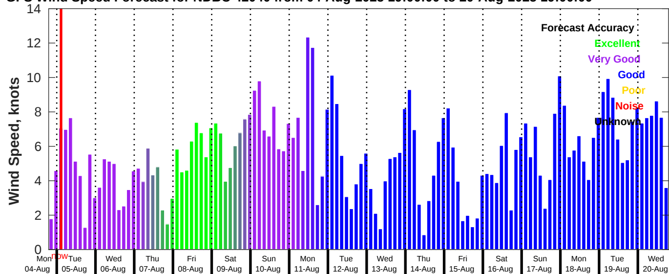
GFS Wind Speed Forecast for NDBC 42040 from 04-Aug-2025 19:00:00 to 20-Aug-2025 19:00:00
