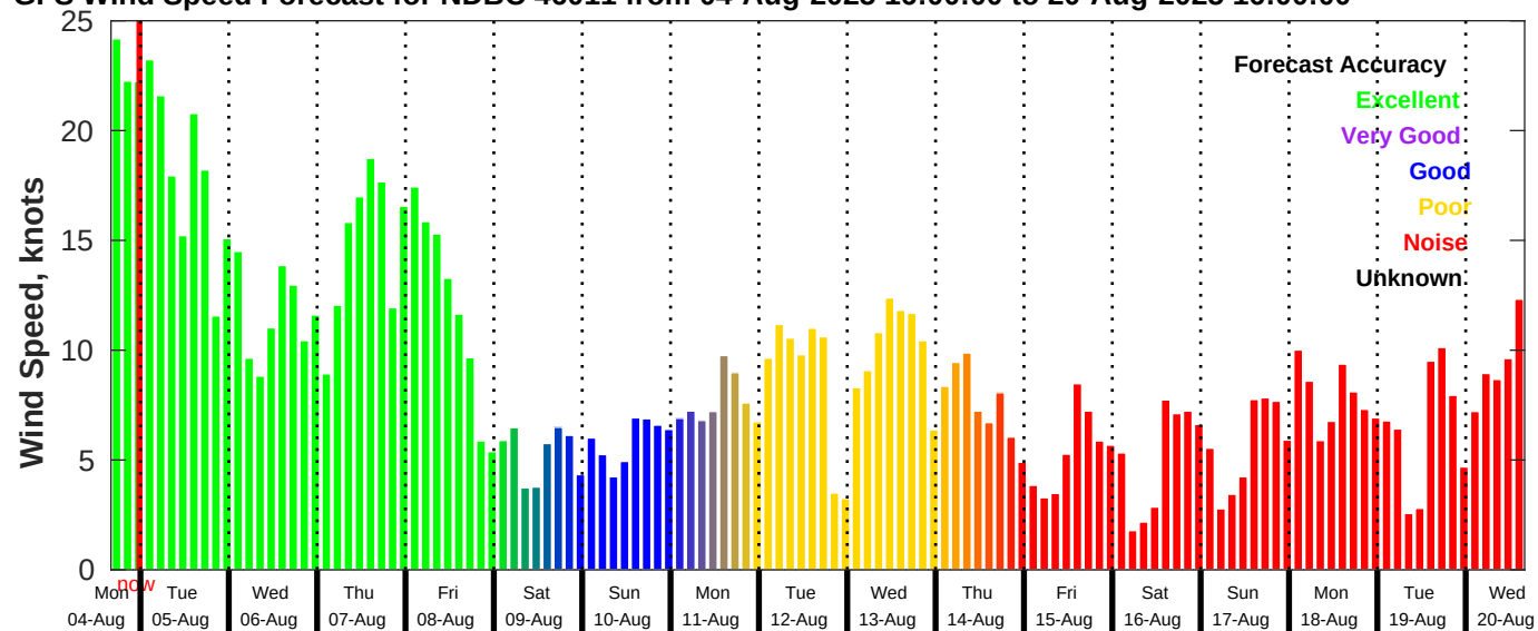
GFS Wind Speed Forecast for NDBC 46011 from 04-Aug-2025 16:00:00 to 20-Aug-2025 16:00:00
