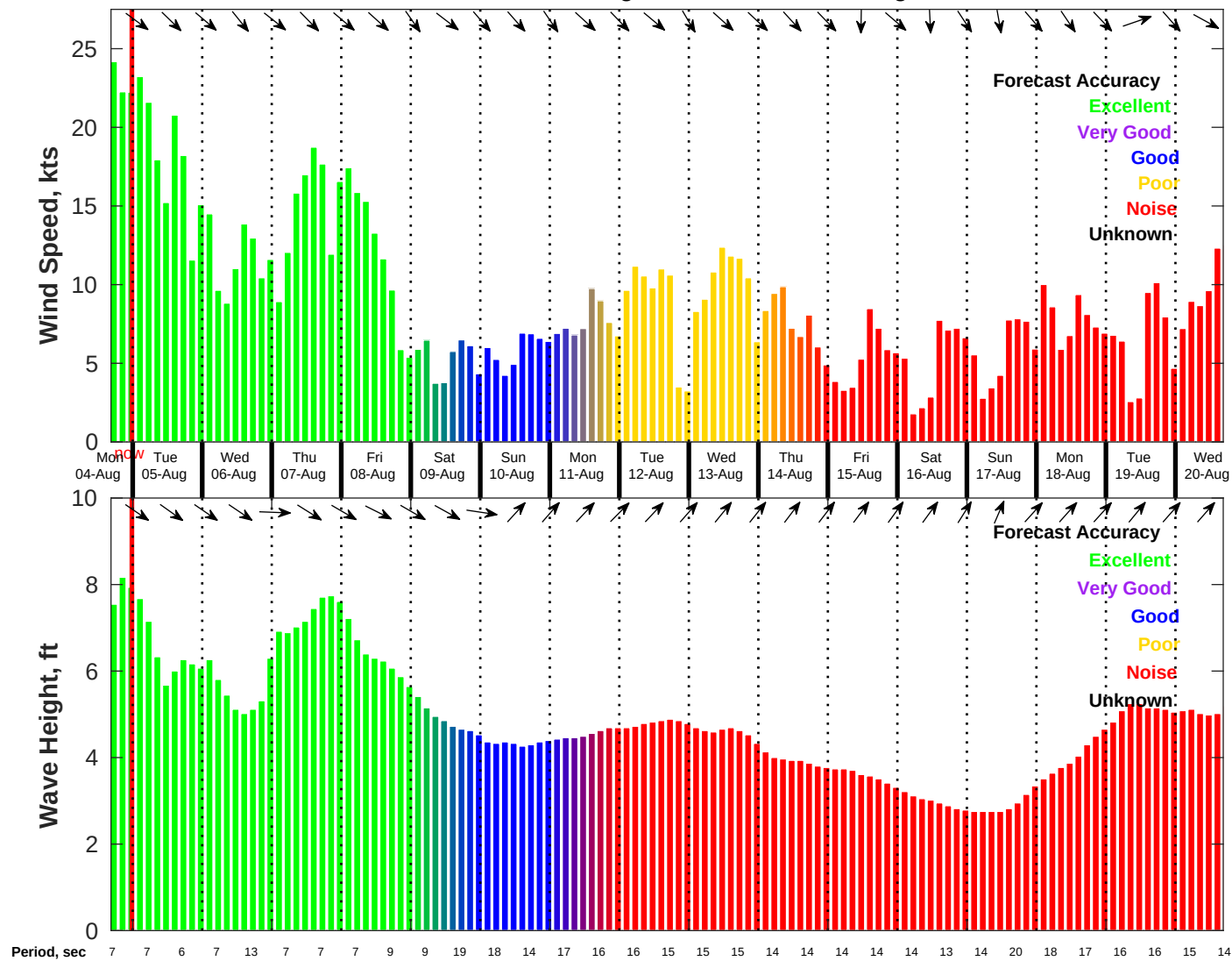
Wind & Wave Forecast for NDBC 46011 from 04-Aug-2025 16:00:00 to 20-Aug-2025 16:00:00
