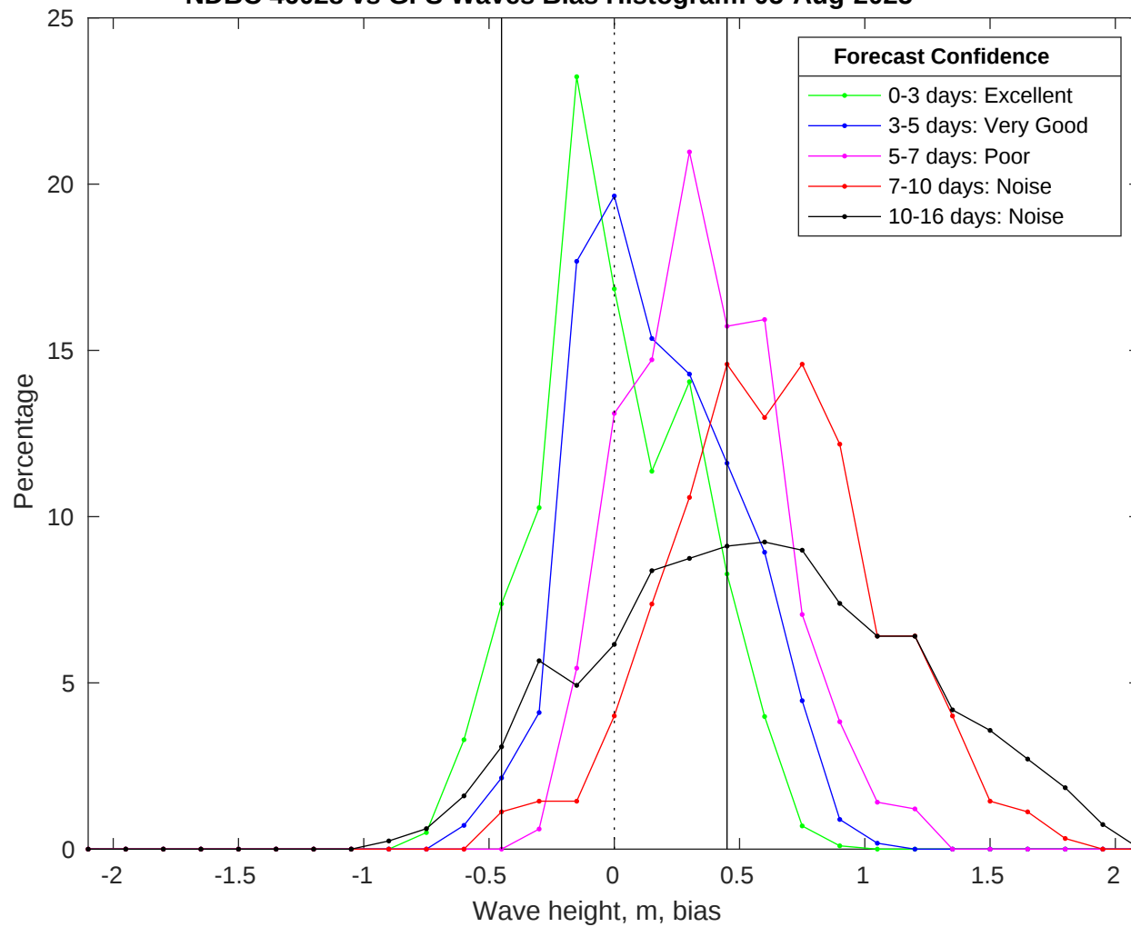
NDBC 46028 vs GFS Waves Bias Histogram: 05-Aug-2025
