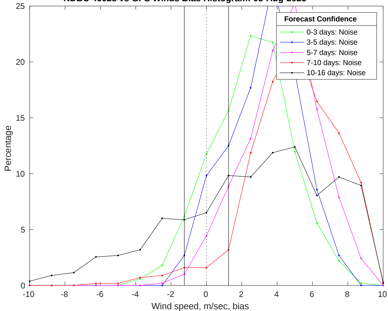
NDBC 46028 vs GFS Winds Bias Histogram: 05-Aug-2025
