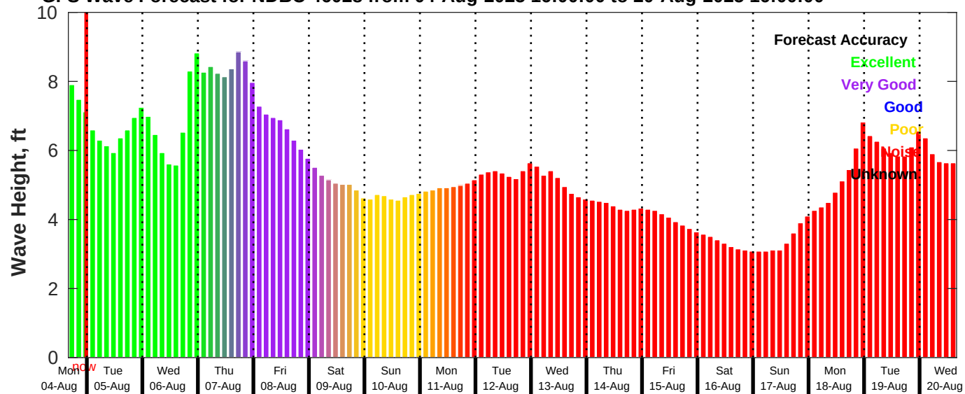
GFS Wave Forecast for NDBC 46028 from 04-Aug-2025 16:00:00 to 20-Aug-2025 16:00:00
