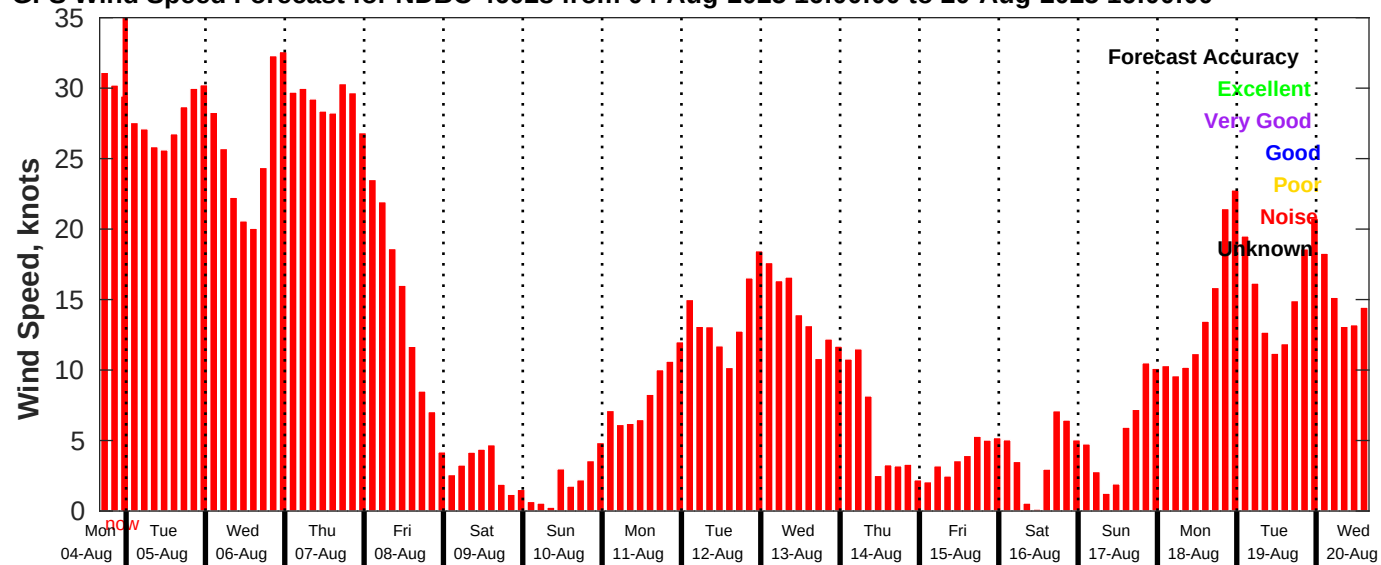
GFS Wind Speed Forecast for NDBC 46028 from 04-Aug-2025 16:00:00 to 20-Aug-2025 16:00:00
