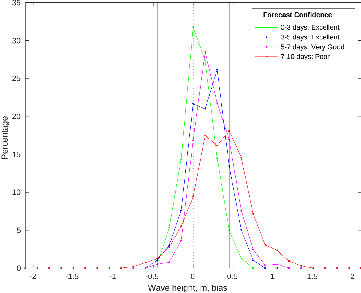
NDBC 46054 vs CMEMS Waves Bias Histogram: 05-Aug-2025
