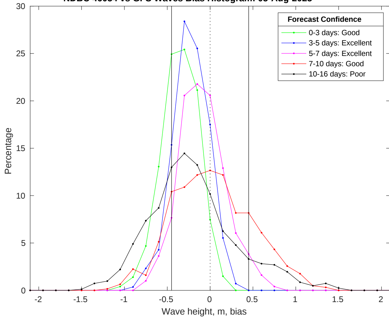
NDBC 46054 vs GFS Waves Bias Histogram: 05-Aug-2025
