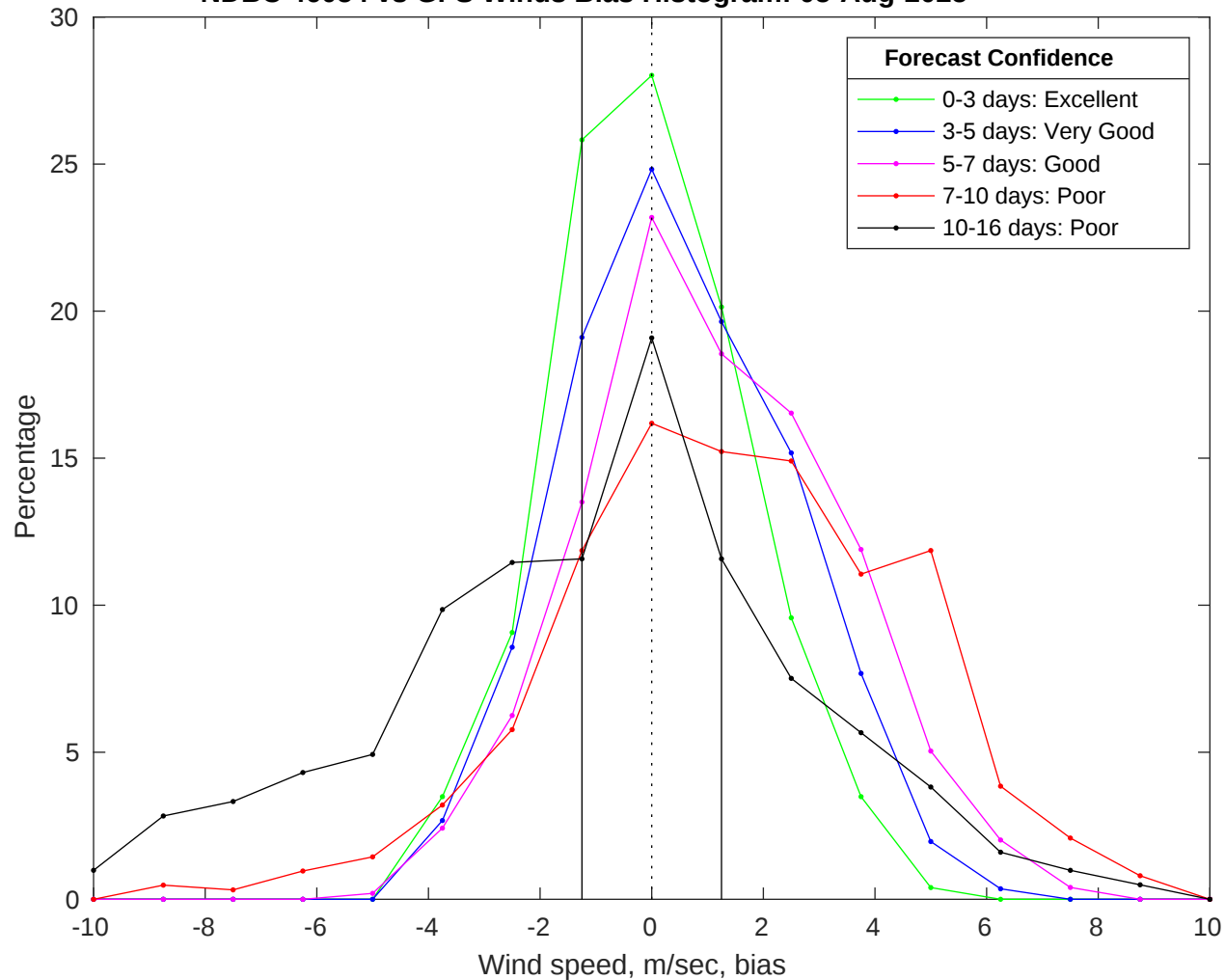
NDBC 46054 vs GFS Winds Bias Histogram: 05-Aug-2025
