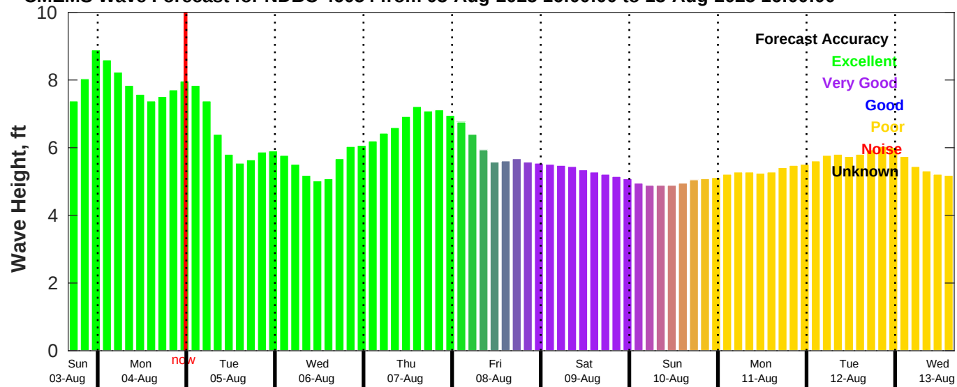
CMEMS Wave Forecast for NDBC 46054 from 03-Aug-2025 16:00:00 to 13-Aug-2025 16:00:00
