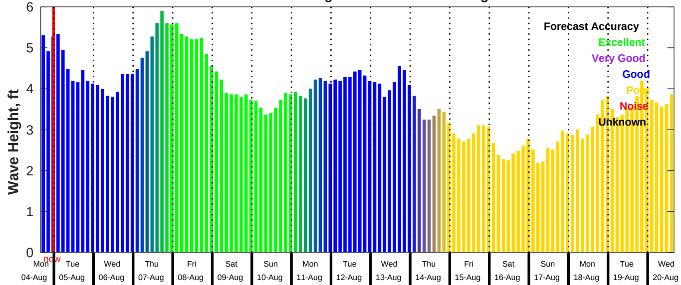
GFS Wave Forecast for NDBC 46054 from 04-Aug-2025 16:00:00 to 20-Aug-2025 16:00:00
