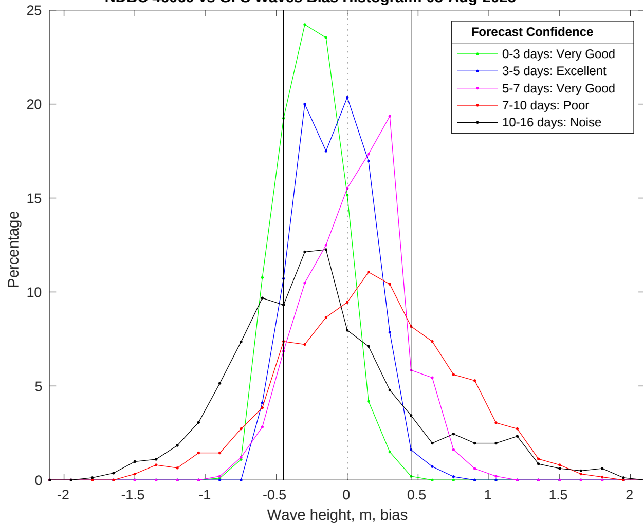
NDBC 46069 vs GFS Waves Bias Histogram: 05-Aug-2025
