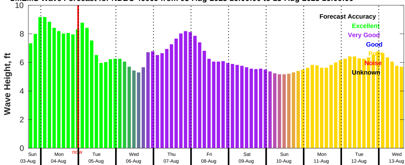
CMEMS Wave Forecast for NDBC 46069 from 03-Aug-2025 16:00:00 to 13-Aug-2025 16:00:00
