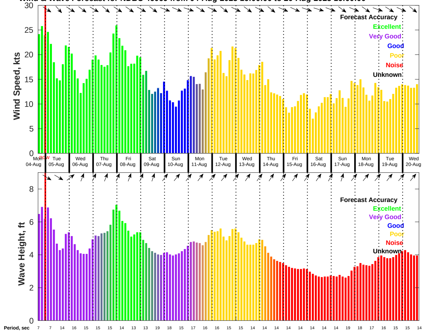
Wind & Wave Forecast for NDBC 46069 from 04-Aug-2025 16:00:00 to 20-Aug-2025 16:00:00
