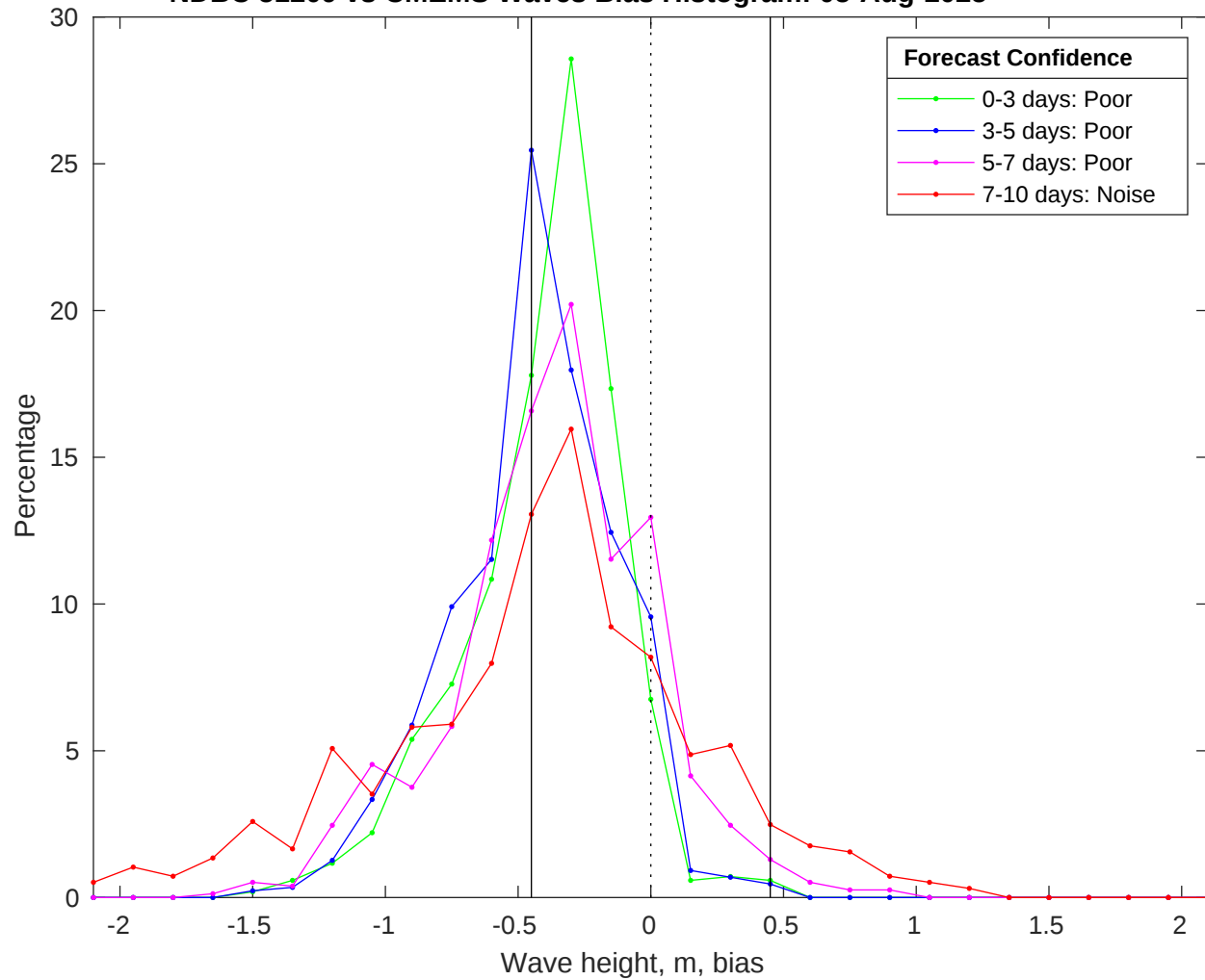
NDBC 51209 vs CMEMS Waves Bias Histogram: 05-Aug-2025
